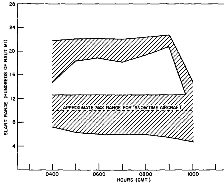
Fig. 4 - Predicted backscatter coverage for October 1968 for an antenna bearing of 55^{\circ}T and an operating frequency of 13 MHz
