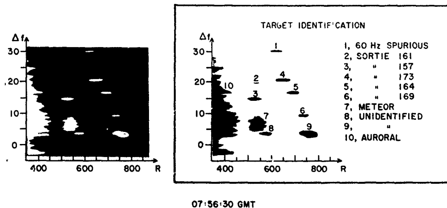
Fig. 11 - Radar doppler-range display with an associated target identification table. The ordinate \Delta f is the doppler frequency in hertz. The abscissa R is slant range in nautical miles.
