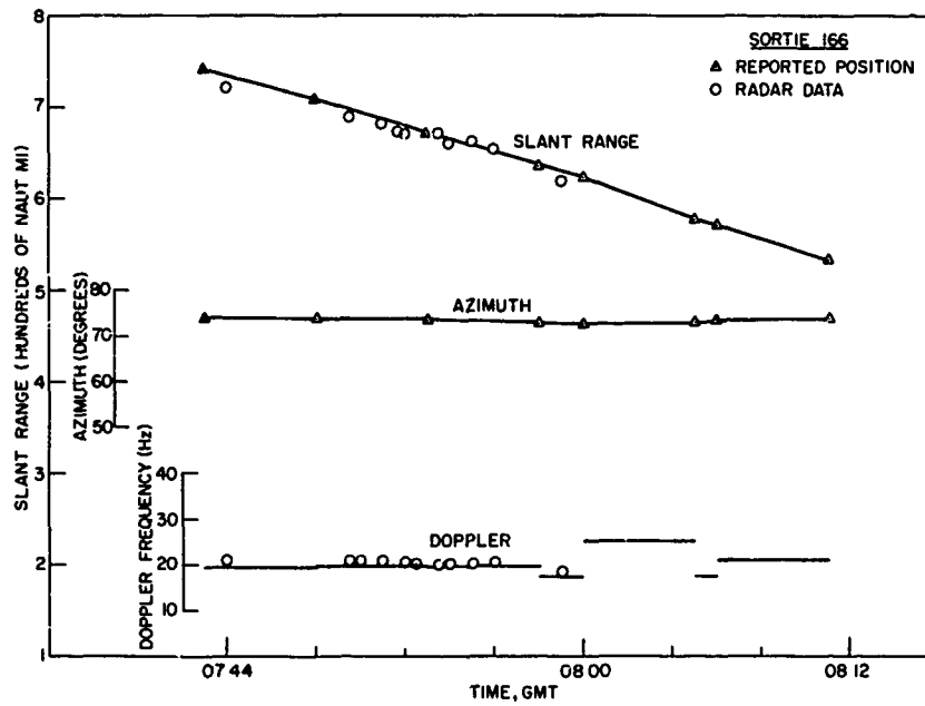
Fig. 16 - Comparison of the reported temporal behavior of Sortie 166 with radar detection data
