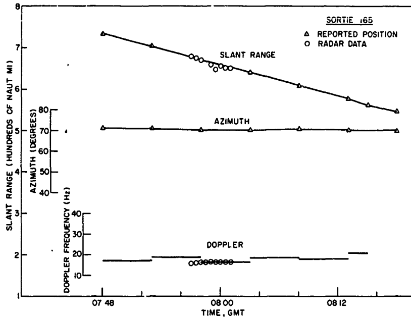
Fig. 15 - Comparison of the reported temporal behavior of Sortie 165 with radar detection data
