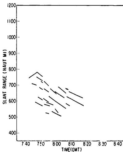
Fig. 9 - Inbound range-time tracks for all inbound aircraft detected
