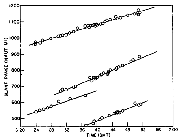
Fig. 7 - Outbound range-time tracks for four selected aircraft
