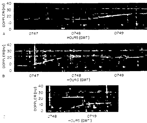
Fig. 21 - Range-gated-doppler-vs-time display reproductions depicting four aircraft doppler tracks. Three aircraft (1, 2, and 4) undergo maneuvers.
