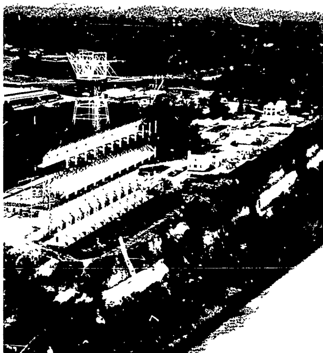
Fig. 1 - OTH facility at NRL's Chesapeake Bay Division. The building at the base and rear of the large array houses transmitter and receiving equipments.
