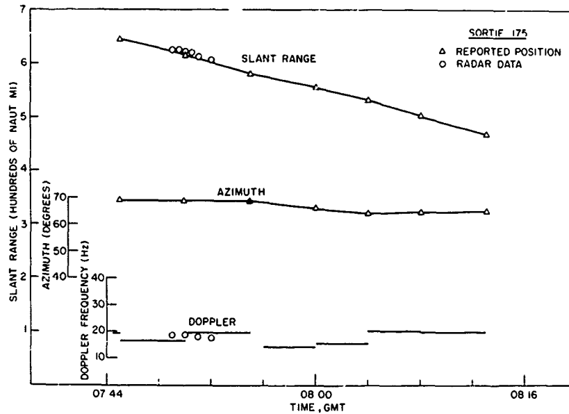
Fig. 19 - Comparison of the reported temporal behavior of Sortie 175 with radar detection data
