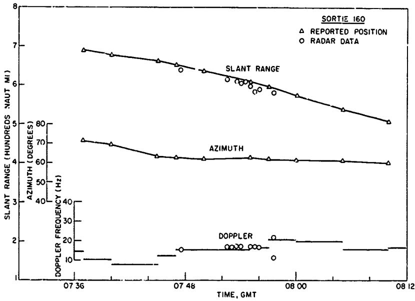
Fig. 13 - Comparison of the reported temporal behavior of Sortie 160 with radar detection data
