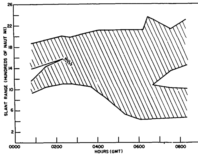
Fig. 6 - Measured backscatter coverage for October 10, 1968, for operation at a bearing of 55°T on 13.575 MHz
