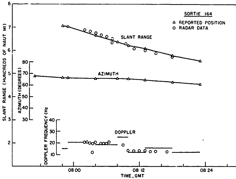
Fig. 14 - Comparison of the reported temporal behavior of Sortie 164 with radar detection data
