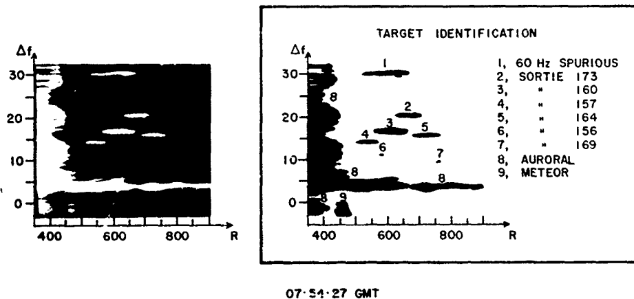
Fig. 10 - Radar doppler-range display with an associated target identification table. The ordinate \Delta f is the doppler frequency in hertz. The abscissa R is the slant range in nautical miles.
