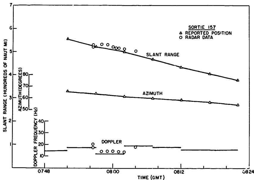
Fig. 12 - Comparison of the reported temporal behavior of Sortie 157 with radar detection data. The azimuth is from the radar.
