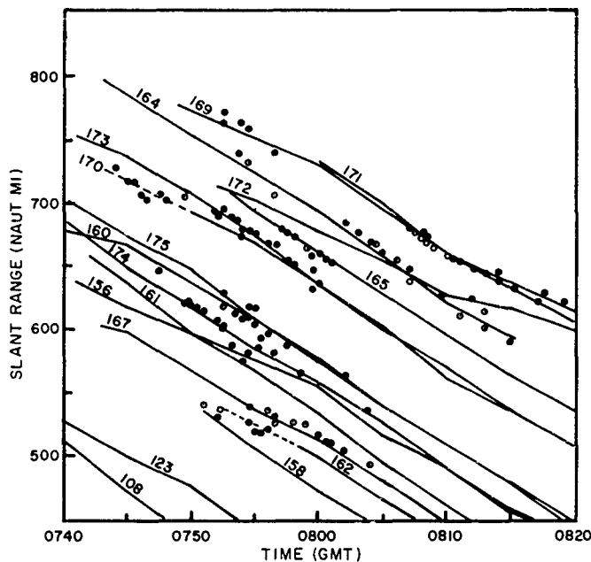
Fig. 20 - Comparison of the reported position tracks of various sorties with radar detection data. All the sorties shown were identified by track comparison except Sorties 108 and 123. Not shown are Sorties 124, 125, 157, and 166.
