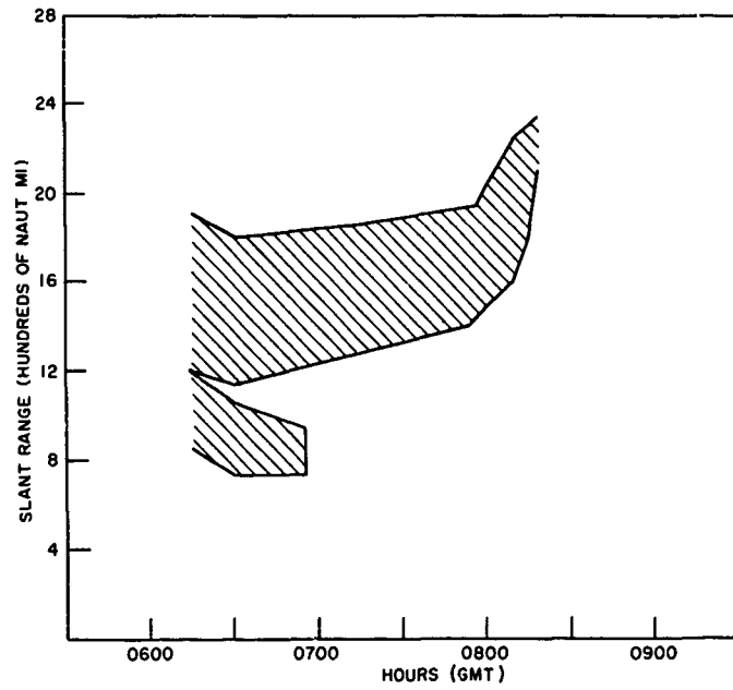
Fig. 5 - Measured backscatter coverage for October 8, 1968, for operation at a bearing of 55°T on 13 MHz nominal
