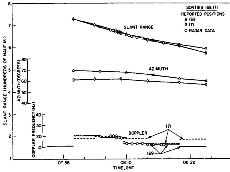
Fig. 17 - Comparison of the reported temporal behavior of Sorties 169 and 171 with radar detection data
